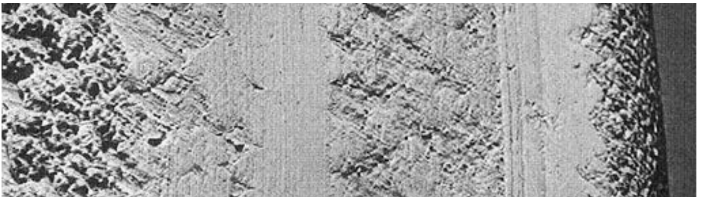
Lubrication with a paste that contains reactive white solid lubricants. Spindle surface after 500,000 motion cycles . Test aborted with spindle being fully intact.
