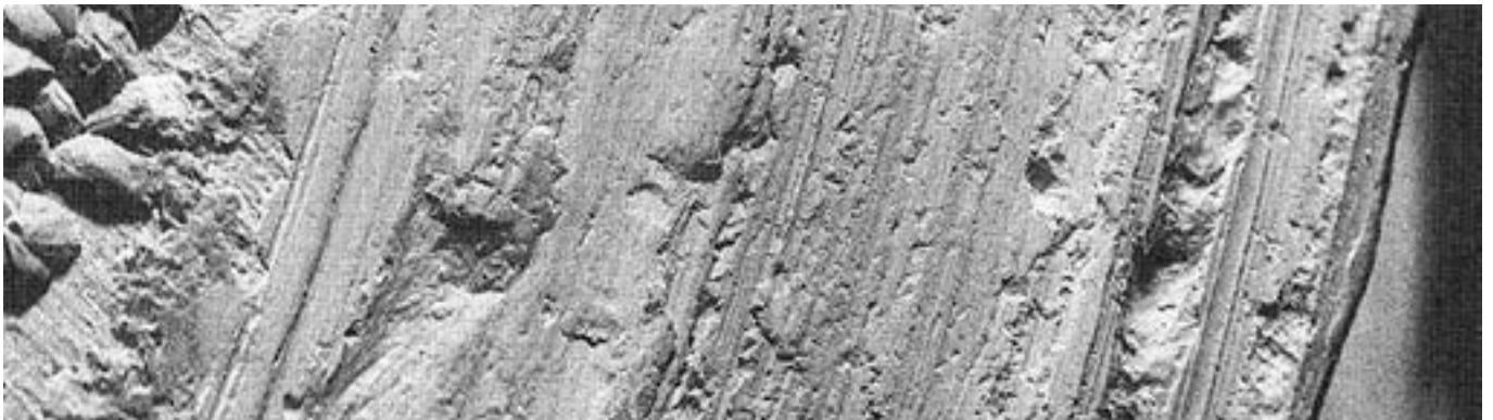
Lubrication with MoS 2 paste. Spindle surface after 35,000 motion cycles . Test aborted, as power consumption of motor too high (torque exceeded).
