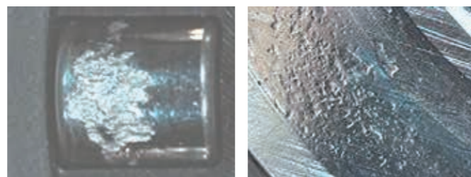
POE ISO VG 170 without additives: pitting, wear
