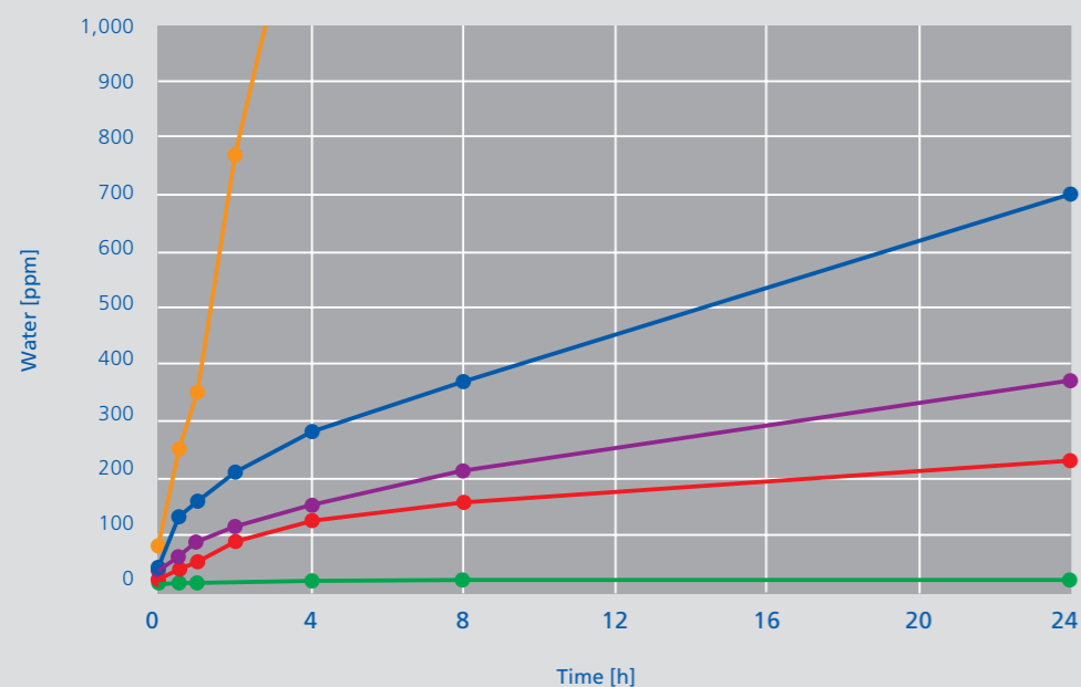
Water absorption (hygroscopicity) of refrigeration oils
