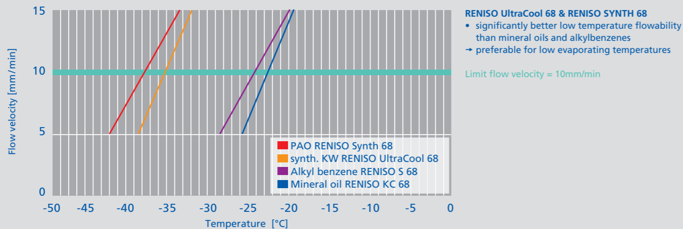
Determination of the flowability of refrigeration oils for NH 3 : U-Tube-Test (DIN 51568) – without refrigerant (low temperature flowability)
