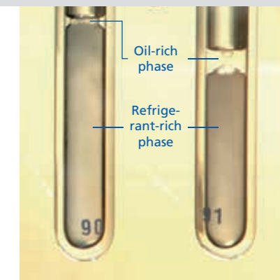
Photo: Phase separation into oil-rich and refrigerant-rich phase (in glass tubes in FUCHS R&D)
