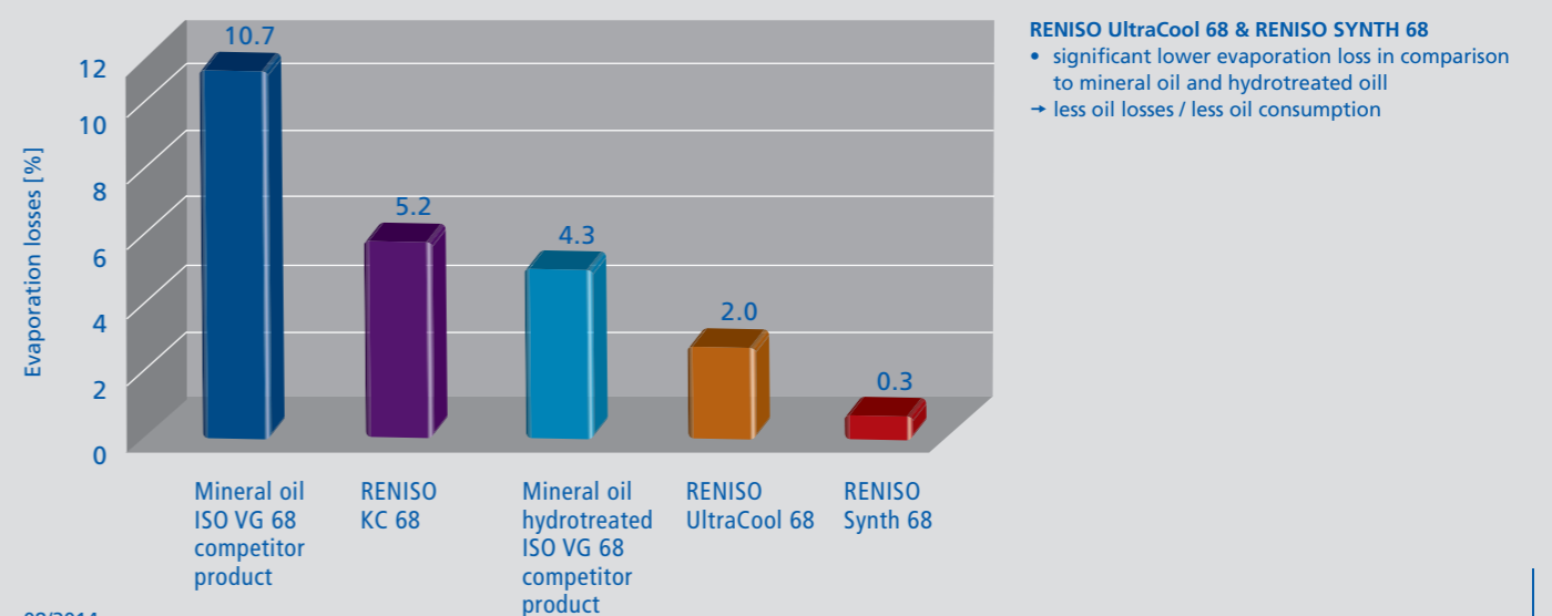
Evaporation losses of refrigeration oils for NH 3 acc. ASTM D972 : 150° / 22h / air flow rate 2l/min
