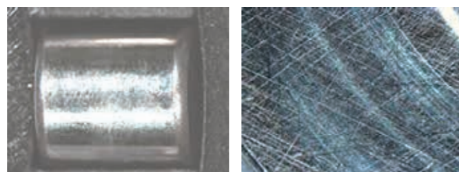
RENISO C 170 E, POE ISO VG 170, with anti-wear additives: no wear
